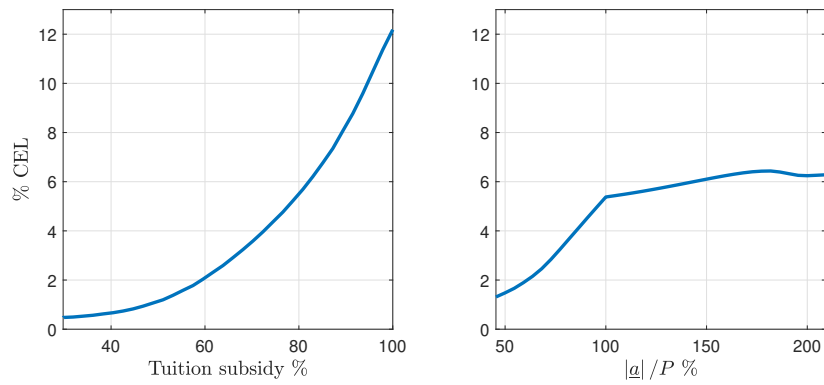
Figure 36: Left - SF to TS for s \in [0.3, 1] - right - SF to ICL1 \underline{a} \in [-2.35, 0.5]
