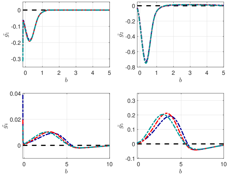
Figure 12: Density difference \tilde{g} = g_{TS} - g_{SF}
