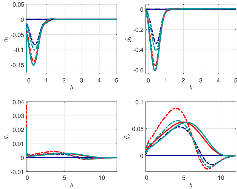
Figure 33: Density difference g_{ICL1} - g_{SF} in partial and general equilibrium. As in Figure(14), dash dotted (solid) lines represent general (partial) equilibrium results and NACL, ICL1 and ICL2 are represented in blue, red and turquoise, respectively.
