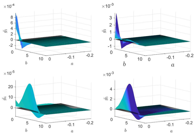
Figure 32: Density difference g_{ICL2} - g_{NICL} in baseline calibration
