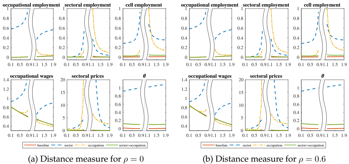
Figure 9: Sensitivity Analysis with respect to \rho
