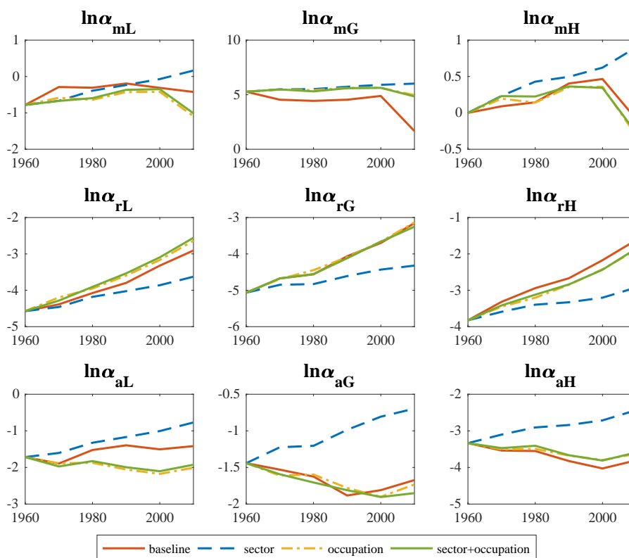
Figure 2: Baseline and counterfactual cell productivity
