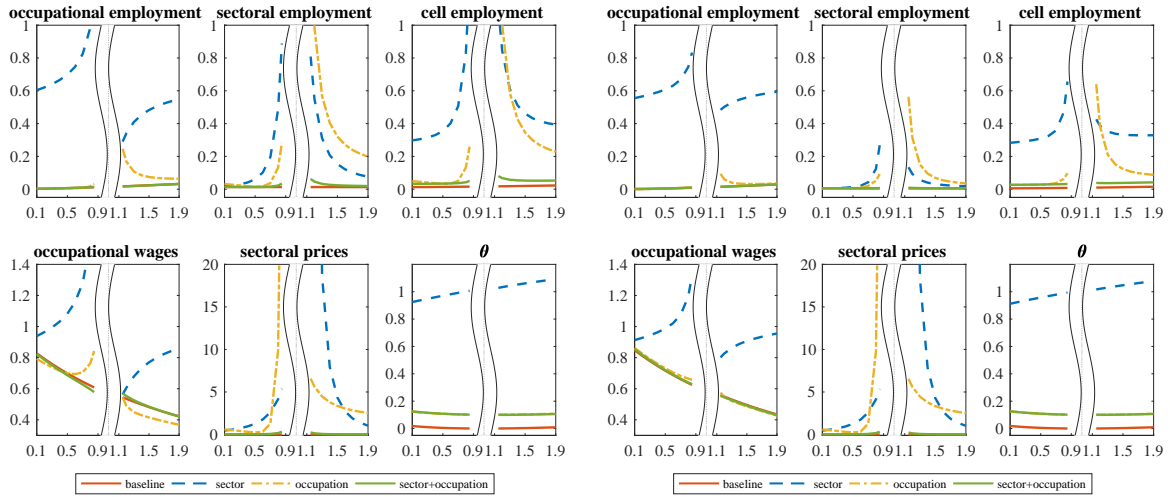
(a) Distance measure for \varepsilon = 0.1
