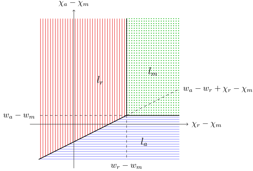
Figure 1: Optimal occupational choice
