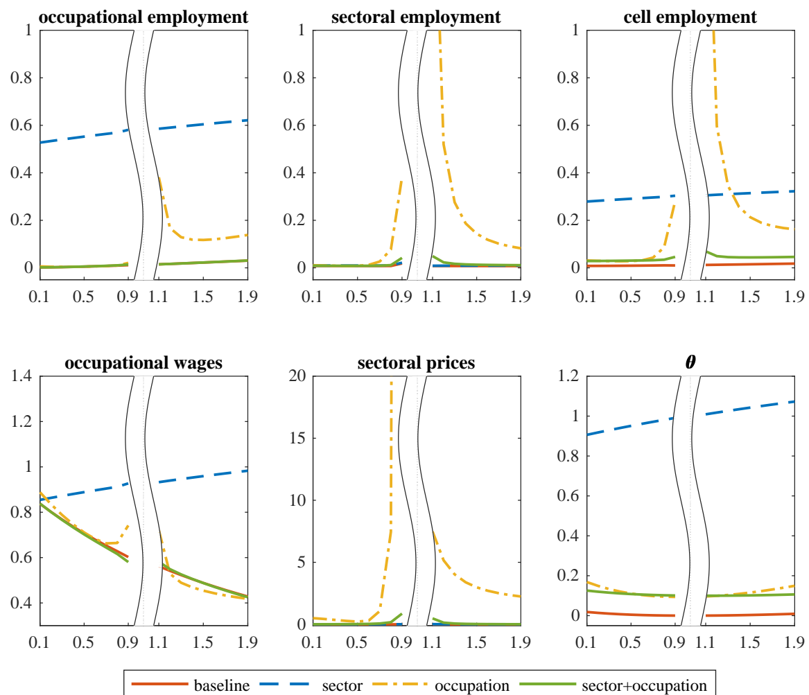
Figure 11: Alternative productivity components' ability to replicate the data
