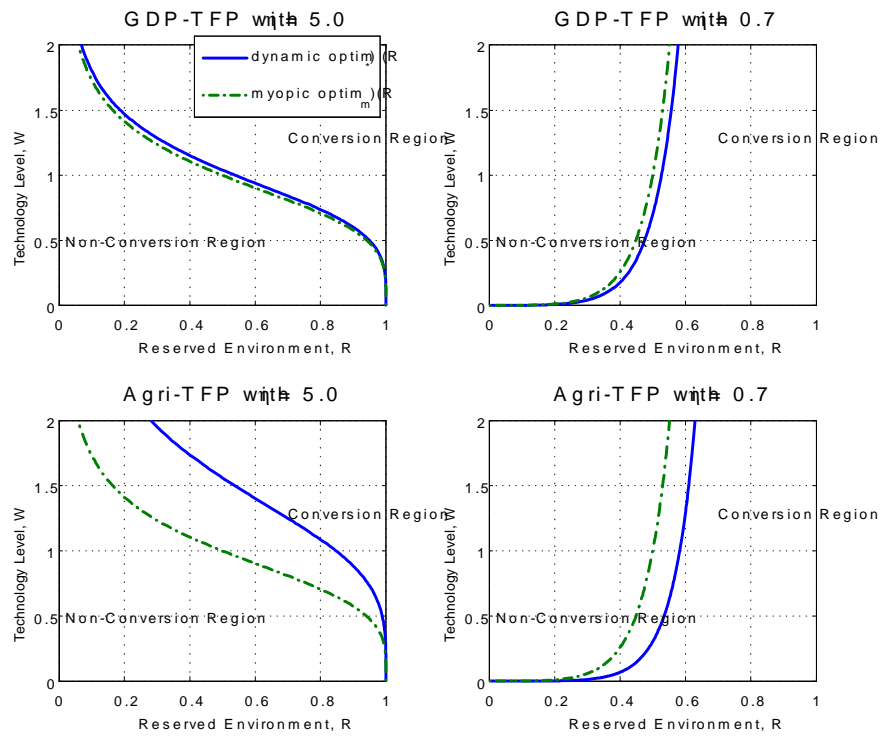
Figure 3: Myopic R_m and Optimal R_* .
