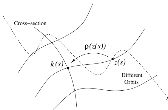
Figure 3: A right moving frame for a curve parametrized by s
