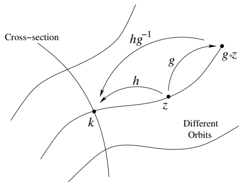
Figure 1: Construction of a right moving frame using a cross-section
